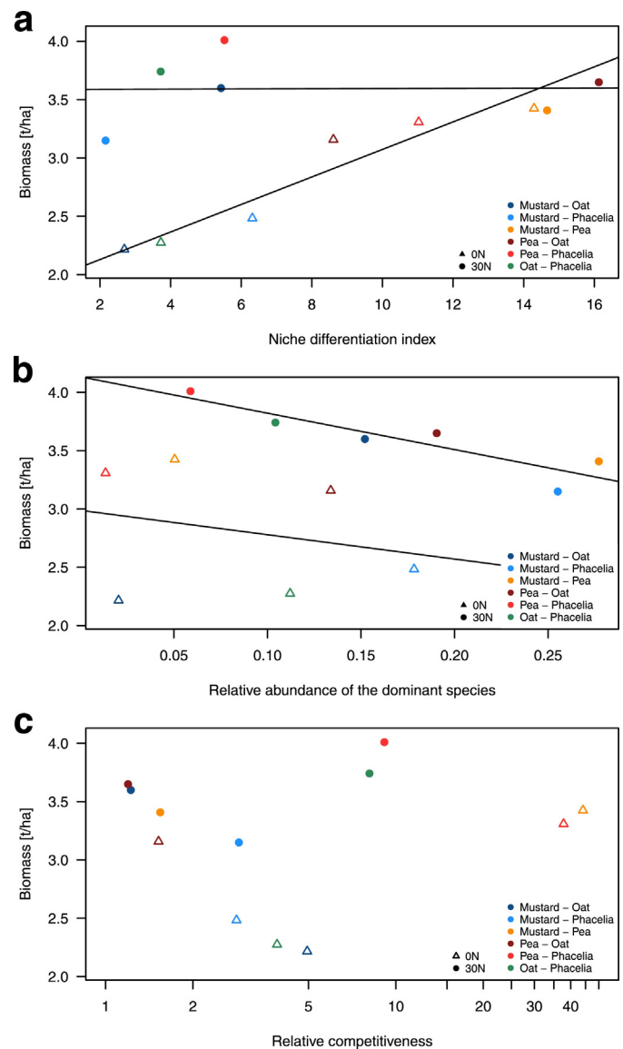
Fig. 6. Shoot biomass of the six mixtures with and without N fertilisation in function of (a) niche differentiation index (NDI), (b) species relative abundance and (c) relative competitiveness (rRC). The relative competitiveness is given on a logarithmic scale.
