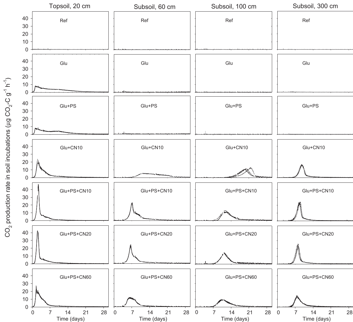
Fig. 1. Rates of \text{CO}_2 production in topsoil (20 cm) and subsoils (60, 100 and 300 cm) in treatments with glucose and nutrients at different C:N:P:S stoichiometry. Data are shown for individual replicates ( n = 3 ) during 30 days of a 42-day incubation period. Treatments: Ref, reference; Glu, glucose; Glu + PS, glucose plus P and S at a C:P:S ratio of 100:1:1; Glu + CN10, glucose plus N at a C:N ratio of 10; Glu + PS + CN10, Glu + PS + CN20, and Glu + PS + CN60, glucose plus N, P and S at C:N:P:S ratios of 100:10:1:1, 100:5:1:1, and 100:1.67:1:1, respectively.
