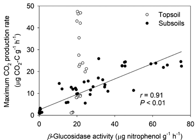
Fig. 3. Correlation between maximum CO 2 production rate during incubation and β-glucosidase activity after incubation for 42 days in topsoil (20 cm; white symbols) and subsoils (60, 100 and 300 cm; black symbols) treated with glucose and nutrients at different C:N:P:S stoichiometry. The correlation was significant for subsoils (line and correlation shown), but not for topsoil ( r = 0.38, P = 0.09).
