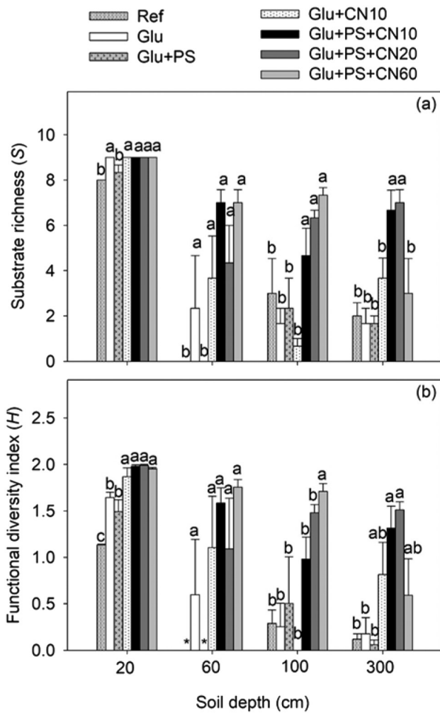
Fig. 4. (a) Substrate richness (S) and (b) Shannon-Weaver diversity index (H) of carbon source utilization in topsoil (20 cm) and subsoils (60, 100 and 300 cm). Utilization of nine divergent carbon sources was assayed with soil from treatments incubated 42 days with glucose and nutrients at different C:N:P:S stoichiometry. Data are mean and standard error ( n = 3 ) with letters indicating significant differences ( P < 0.05 ) between treatments within the same soil depth. Asterisks shown in panel b indicate that H was not calculated when S was zero. Treatments: Ref, reference; Glu, glucose; Glu + PS, glucose plus P and S at a C:P:S ratio of 100:1:1; Glu + CN10, glucose plus N at a C:N ratio of 10; Glu + PS + CN10, Glu + PS + CN20, and Glu + PS + CN60, glucose plus N, P and S at C:N:P:S ratios of 100:10:1:1, 100:5:1:1, and 100:1.67:1:1, respectively.
