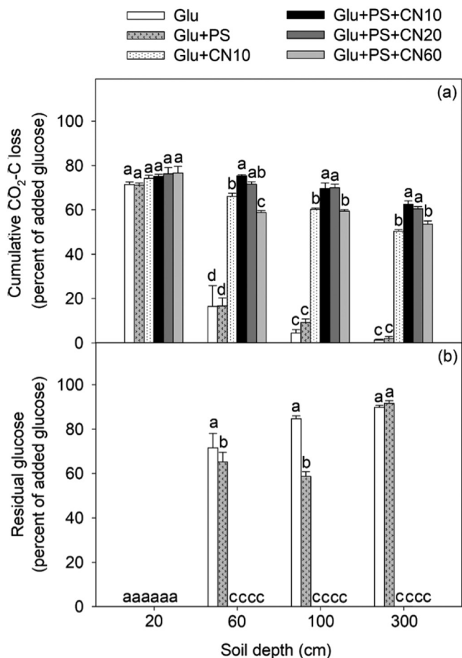
Fig. 2. (a) Cumulative CO 2 -C loss and (b) remaining labile (residual) glucose content in topsoil (20 cm) and subsoils (60, 100, and 300 cm) after incubation for 42 days with glucose and nutrients at different C:N:P:S stoichiometry. Data are mean and standard error ( n = 3) with letters indicating significant differences ( P < 0.05) between treatments within the same soil depth. Treatments: Glu, glucose; Glu + PS, glucose plus P and S at a C:P:S ratio of 100:1:1; Glu + CN10, glucose plus N at a C:N ratio of 10; Glu + PS + CN10, Glu + PS + CN20, and Glu + PS + CN60, glucose plus N, P and S at C:N:P:S ratios of 100:10:1:1, 100:5:1:1, and 100:1.67:1:1, respectively.
