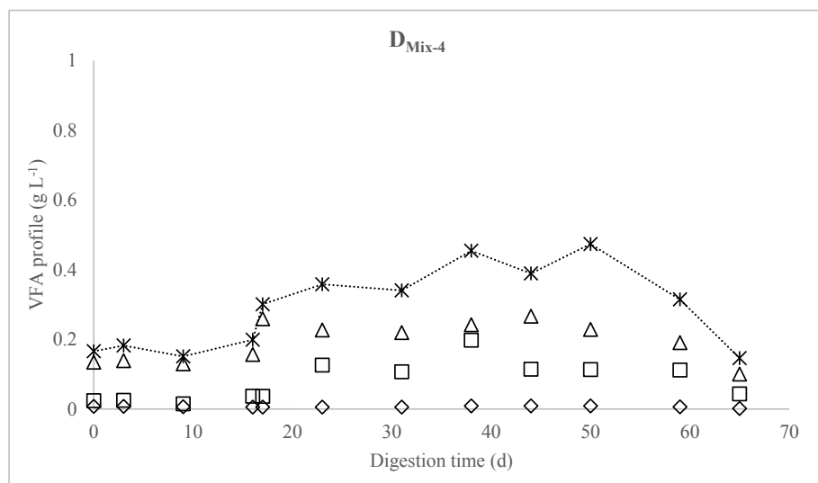
Fig. 5. VFA profile (total and individual VFA) of effluent from (a) D Mix-4 and (b) D Lu-4 .
