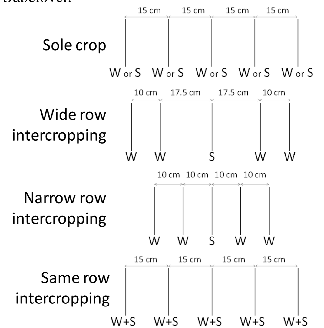
Figure 1. Layout of wheat-subclover intercropping systems and monocultures. W = durum wheat; S = Subclover.
