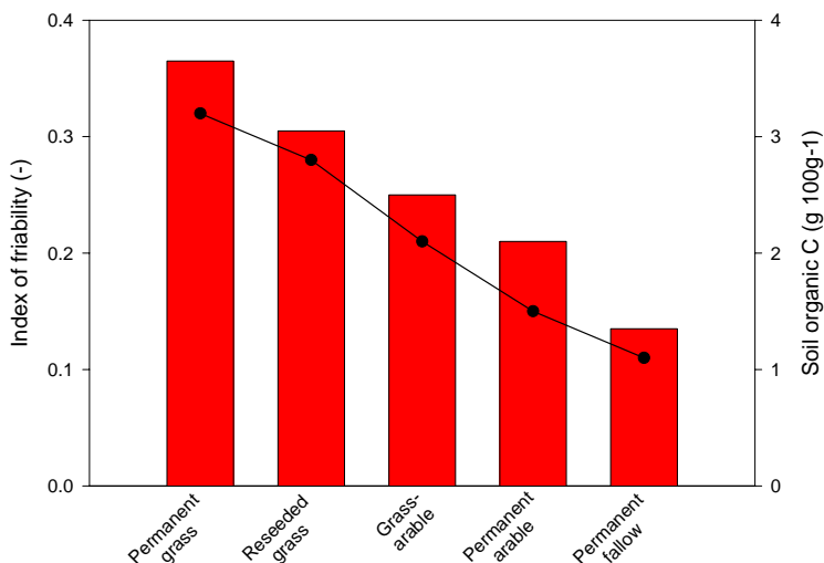
Figure 6.2. Index of friability calculated from tensile strength of dry aggregates (bars) and soil organic C (dot symbols and line). The friability index is calculated as \frac{1}{2} \times F1 , where F1 is the index presented by Watts & Dexter (1997) in their study of aggregates from plots of the long-term Rothamsted rotation experiments.
