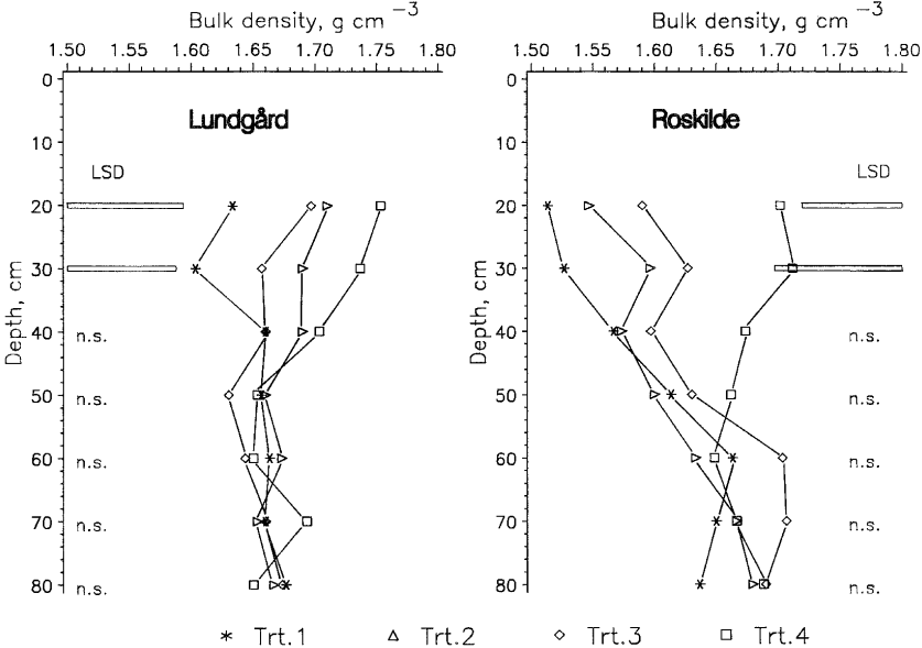
Figure 5.5. Soil bulk density measured with a gamma transmission technique one year after compaction treatments with a dump truck (~5 tonnes wheel load) for two Danish soils (Lundgård: coarse sandy soil; Roskilde: loamy sand). Trt. 1: control (no compaction); Trt. 2: one pass on topsoil; Trt. 3: four passes on topsoil; Trt. 4: four passes on exposed plough bottom. Reproduced from Schjønning & Rasmussen (1994).
