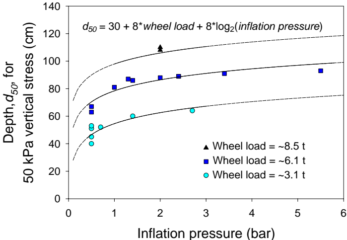
Figure 5.13. Symbols show Söhne-predicted maximum depth of 50 kPa vertical stress in relation to wheel load and tyre inflation pressure. Based on Söhne simulations on average stress distributions for each of 20 tested combinations of tyre type, wheel load and inflation pressure. The lines show the predictions of the suggested, approximate equation (the ‘8-8 rule’; Equation 1). Notice that the model requires wheel load and inflation pressure in units of tonnes and bars, respectively. Reproduced from Schjøning et al. (2006b).
