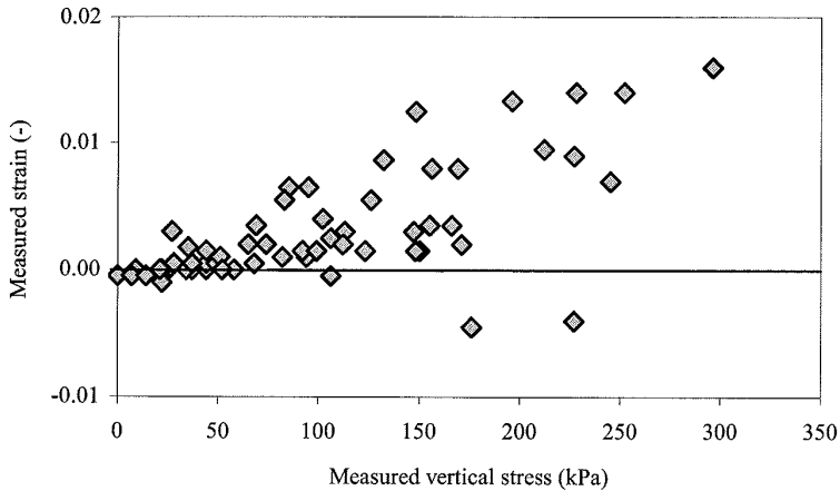
Figure 5.12. Measured strain (relative deformation of given soil layer) as related to the measured vertical stress for a number of soil compaction tests in Sweden and Denmark (Keller, 2004).
