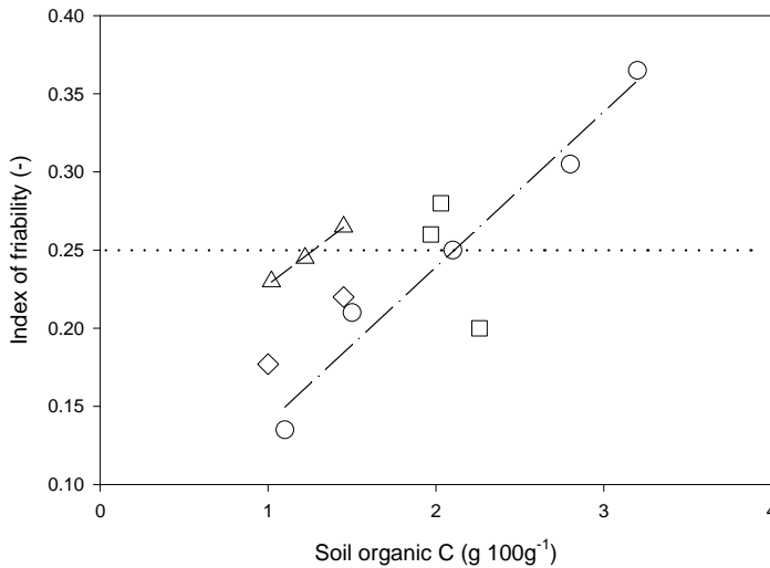
Figure 6.14. Index of friability calculated from tensile strength of dry aggregates as related to the soil organic C for a range of soils. Circles: soil from the Rothamsted experiment (Fig. 6.2), triangles: soil from the Askov experiment, squares: soil from Danish forage cropping systems, diamonds: soil from Danish cash crop systems. The index of friability for the Danish locations was calculated as the F3 index (Dexter, 2004b), while that for the English location was calculated as \frac{1}{2} \times F1 . Please consult Dexter (2004b) for an explanation that this makes the indices comparable. The dash-dot line indicate linear regression of the Rothamsted data, while the dash line indicate regression for the Askov data (Watts & Dexter, 1997; Munkholm et al., 2001a, 2002; Schjønning, unpublished data).
