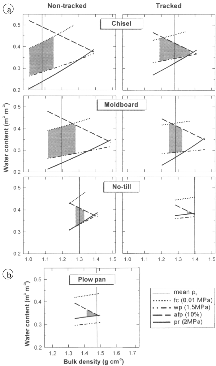
Fig. 5.4. The Least Limiting Water Range (LLWR) concept for (a) the topsoil and (b) the plough pan of a clay loam. Crop growth is constricted at water contents below and above the limits indicated by the shaded areas. Four limiting water contents for soil functions are identified: \theta_{fc} , \theta_{wp} , \theta_{afp} and \theta_{pr} , representing field capacity (fc), wilting percentage (wp), 10% air-filled pore space (afp), and 2 MPa penetration resistance (pr), respectively. Reproduced from Betz et al. (1998).
