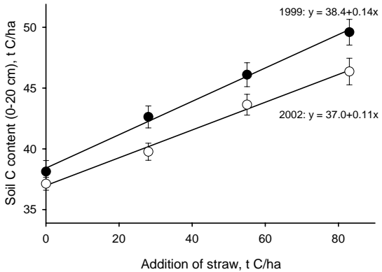
Figure 6.6. Soil C content (0-20 cm) one year (1999) and four years (2002) after the last addition of straw as a function of the amount of C added in straw in the experimental period 1989-1998. See Figure 6.5 for additional explanation (Thomsen & Christensen, 2004).
