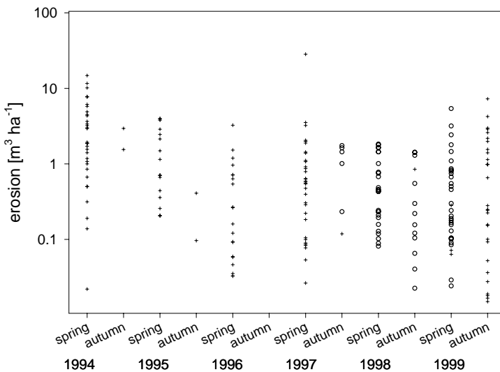
Figure 7.1. Measured rill erosion rates in spring and autumn on 213 slope units in Denmark (Djurhuus et al., 2007).
