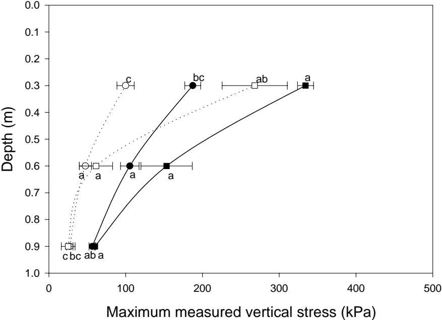
Figure 5.9. Maximum vertical stress measured in the soil profile (0.3, 0.6 and 0.9 m depths) for four compaction treatments in a Stagnic Luvisol at a water content of field capacity (white circles: 800/50R34 - 30 kN; black circles: 800/50R34 - 60 kN; white squares: 560/45R22.5 – 30 kN; black squares: 560/45R22.5 – 60 kN). Error bars represent standard errors. Different letters indicate significant differences between treatments (P=0.05). Reproduced from Lamandé & Schjønning (2009b).
