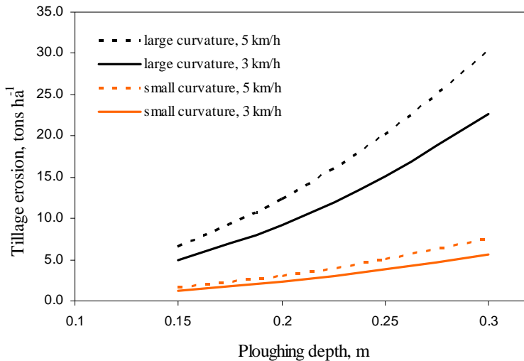
Figure 8.2. Predicted tillage erosion rates for mouldboard ploughing as a function of tillage depth, speed and topography. The tillage direction is parallel to the aspect and the soil bulk density 1400 \text{ kg m}^{-3} . Based on Van Oost et al. (2006).
