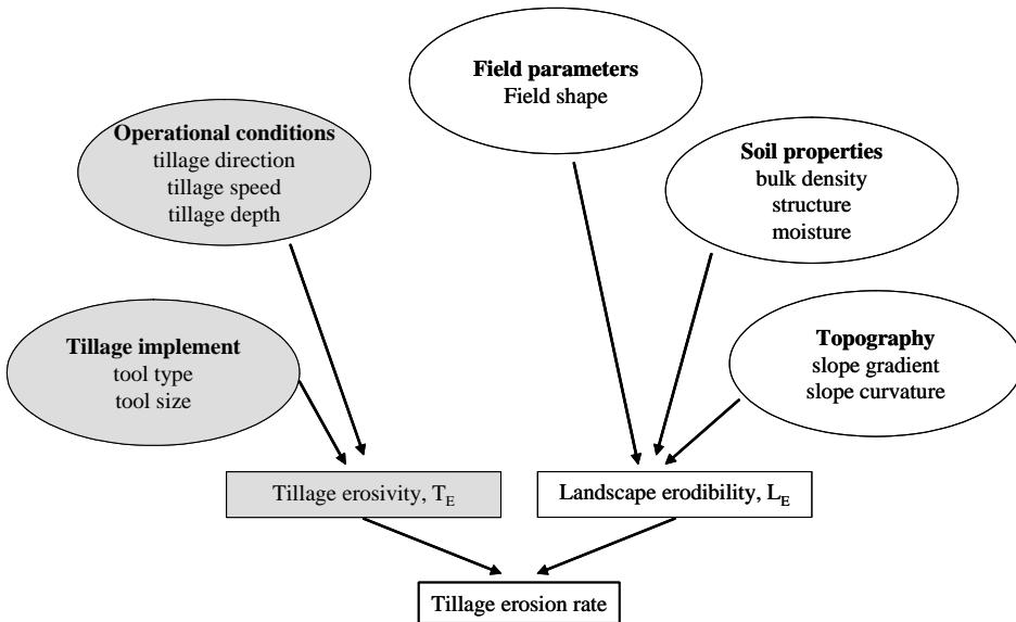
Figure 8.1. Factors affecting tillage erosion. The process of tillage erosion can be seen as a function of the erosivity of a given tillage operation ( T_E ) and the erodibility of the cultivated landscape ( L_E ). This simple general concept is the basis for the following discussion. Adapted from Lobb et al. (1999).
