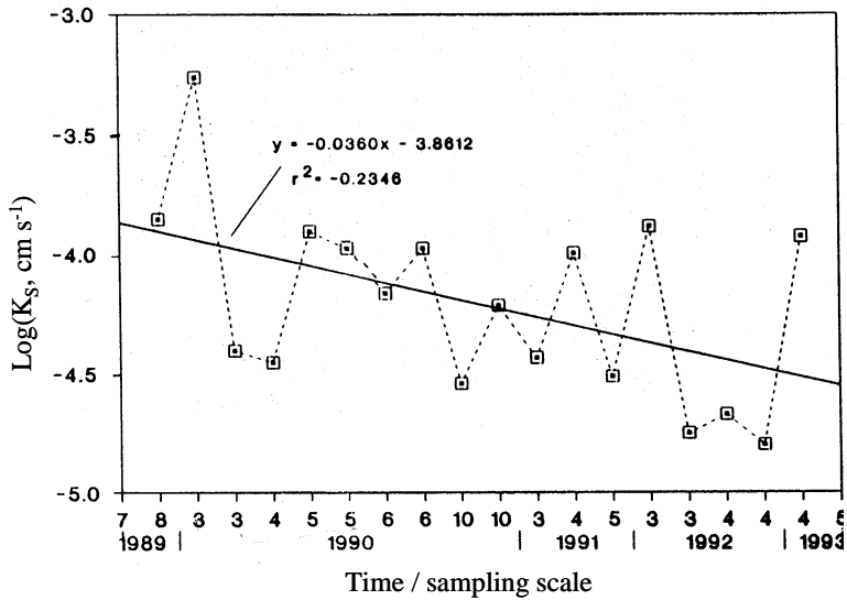
Figure 5.6. Saturated hydraulic conductivity, K_s , of soil at 40 cm depth as measured at intervals in a four-year period with heavy traffic. Please note that the abscissa is not a traditional time axis. (Semmel, 1993; Horn et al., 1995).
