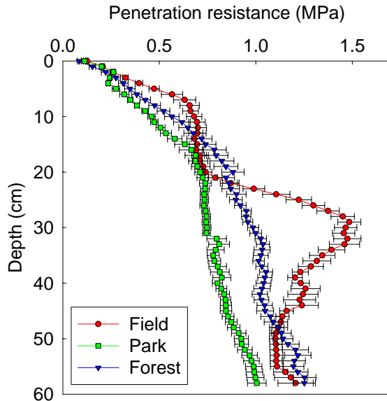
Figure 5.1. Cone penetration resistance measured at Barritskov Manor (loamy soil) in a non-trafficked park, a forest and in an agricultural field. Bars denote standard deviation (n=40) (Schjønning et al., 2000b).
