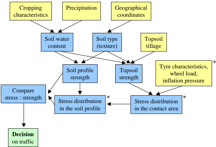
Figure 5.15. Route diagram illustrating the information flow in the planned decision support system 'JORDVÆRN online' allowing an evaluation of the sustainability of an intended traffic event on a specific field in Denmark. Please consult text for explanation of details. The boxes marked with an asterisk constitute the existing web tool ( www.planteinfo.dk , sheet 'Jord').
